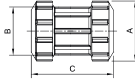
Racor acoplamiento recto con bridas Straight coupling double connector with flanges
