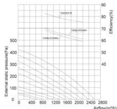
RCH-2000 Performance Chart
