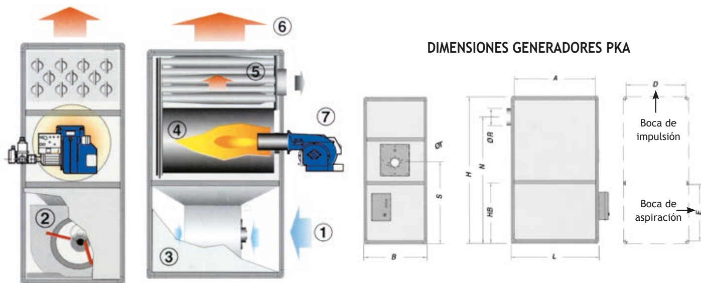
Vista Frontal
