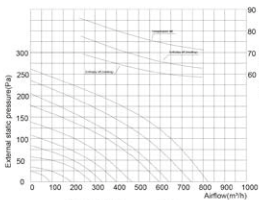
RCH-650 Performance Chart
