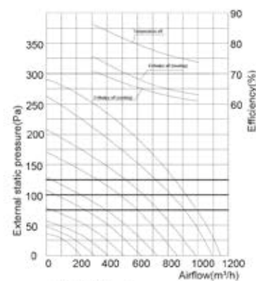
RCH-800 Performance Chart
