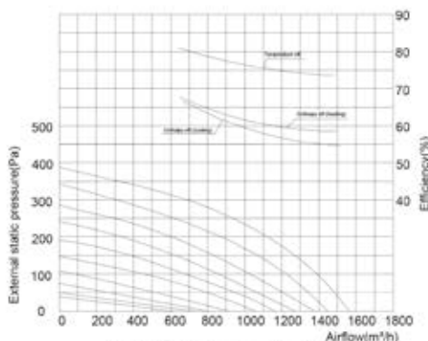
RCH-1300 Performance Chart
