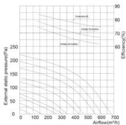
RCH-500 Performance Chart
