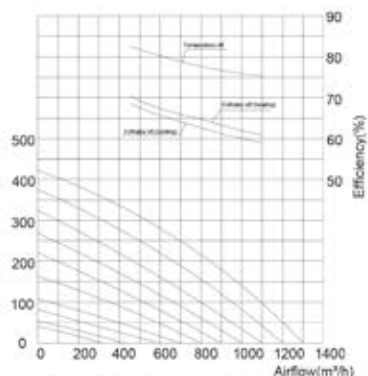
RCH-1000 Performance Chart
